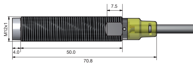
Fig. 9 Long body, non-flush version, cable
