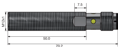
Fig. 10 Long body, flush version, plug
