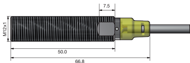
Fig. 8 Long body, flush version, cable
