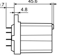
062.10 with relay
