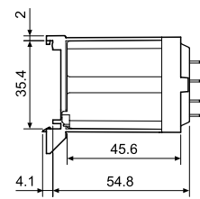
062.07 with relay
