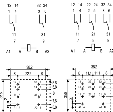
62.22 Copper side view
