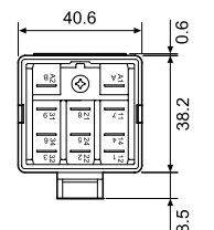
062.07 with relay
