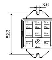
062.05 with relay
