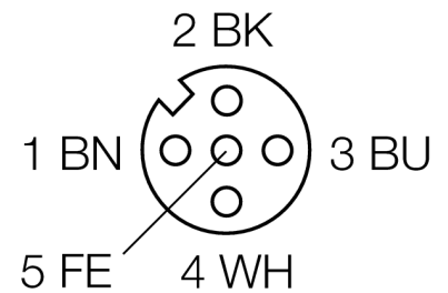
pin configuration left
